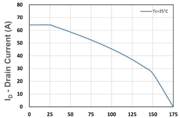
T_j - Junction Temperature ( ^{\circ}C ) Figure 10. Drain Current
