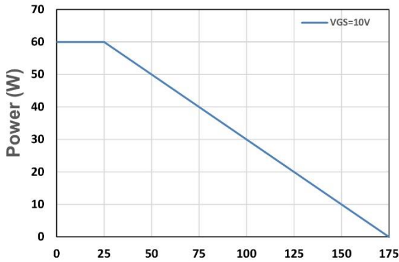
T_c - Junction Temperature ( ^{\circ}C ) Figure 9. Power Dissipation
