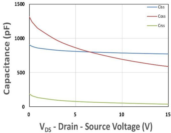
Figure 7. Capacitance
