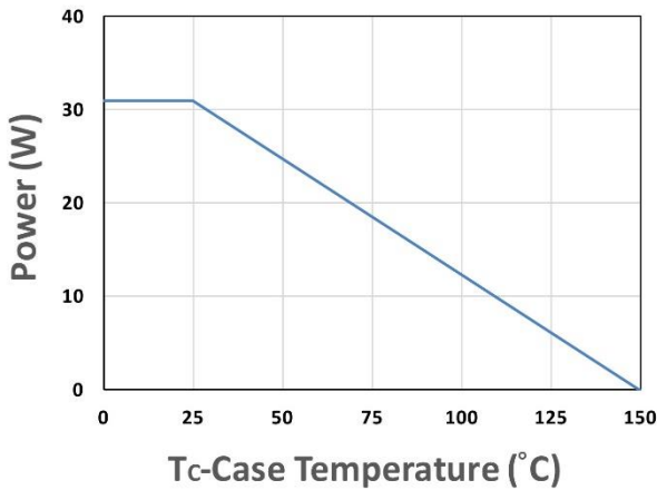
Figure 9. Power Dissipation
