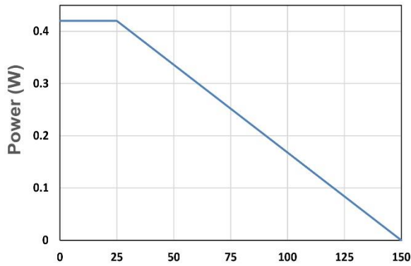
T_A - Junction Temperature ( ^{\circ}\text{C} ) Figure 9. Power Dissipation
