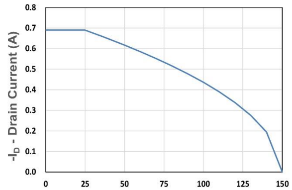
T_A - Junction Temperature ( ^{\circ}\text{C} ) Figure 10. Drain Current
