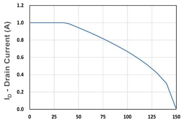
T_A - Junction Temperature (°C) Figure 10. Drain Current
