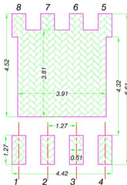
Suggested Pad Layout(Unit:mm)
