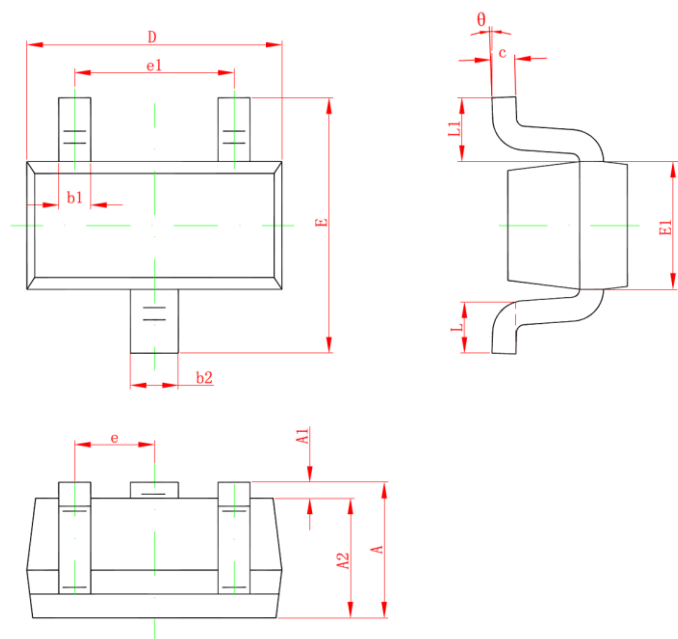
Suggested Pad Layout(Unit:mm)
